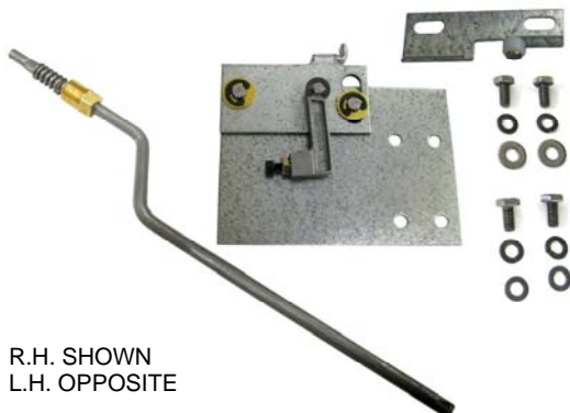
CLU9-0115L/R LOCKING ASSEMBLY,LWZ-2 CLUTCH 36" ROD WITH STANDARD CAM
