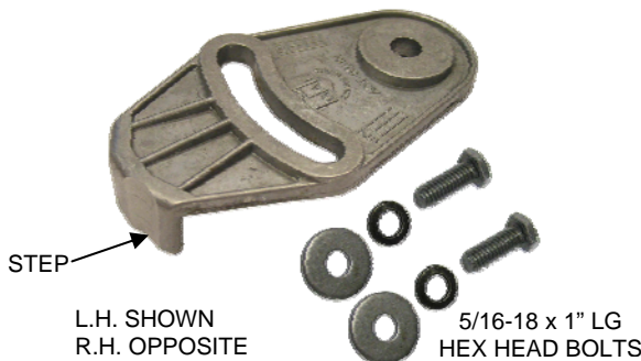
CLU9-0238L/R CAM, LW2-LRC & LWZ-2-LRC CLUTCH ACTUATING
