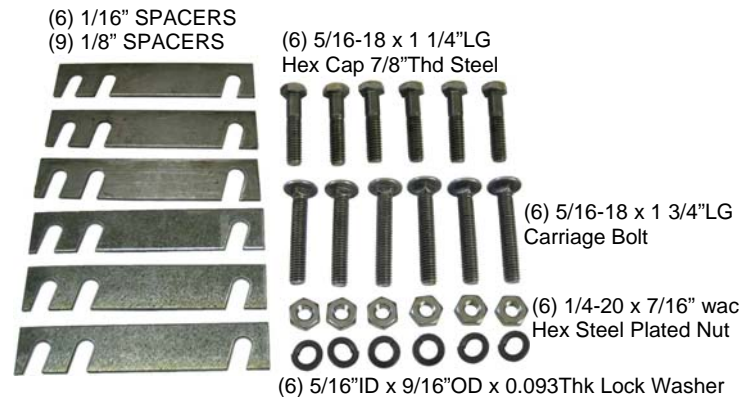
CLU9-0046N HARDWARE, CLUTCH MOUNTING LWZ-2-LOW & LWZ-2-LRC LOW CLUTCHES
